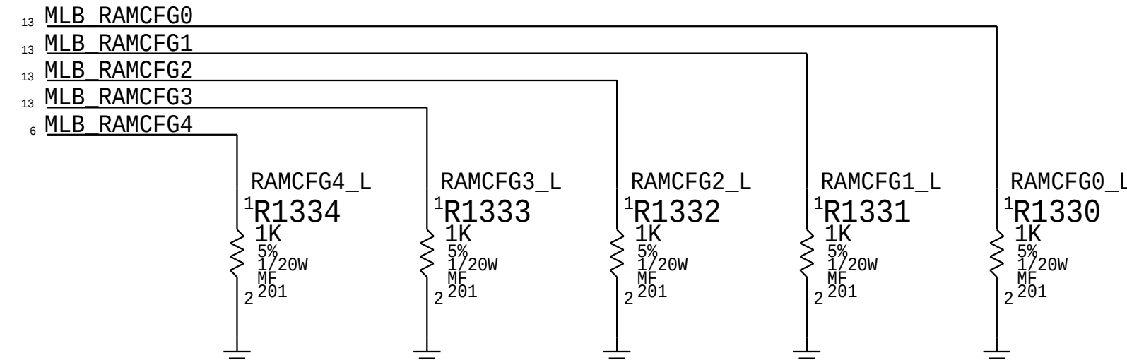
MEMORY CONFIGURATION STRAPS.
